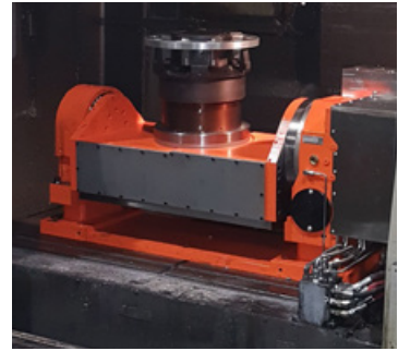
NC AXLE (CUTTING)
