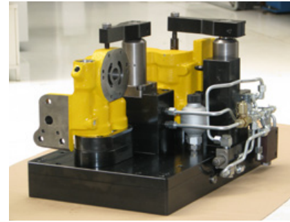
CLAMPING MACHINERY (CUTTING)
