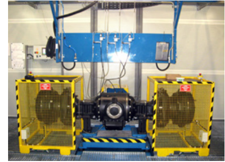
FINAL INSPECTION TEST MACHINE (VEHICLE INDUSTRY)
